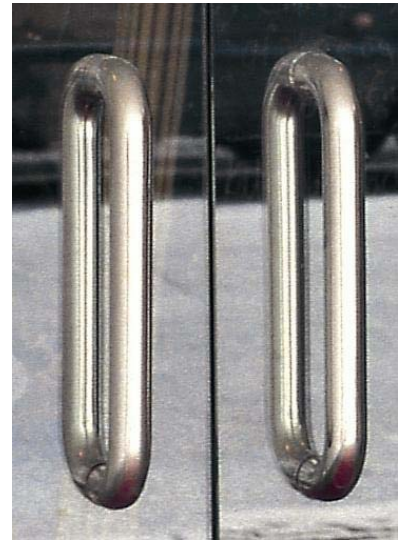
Pull # 15.930 25 x 70 x 300 mm Mounted through glass using glass fittings #15.00G and through bolts #15.010
