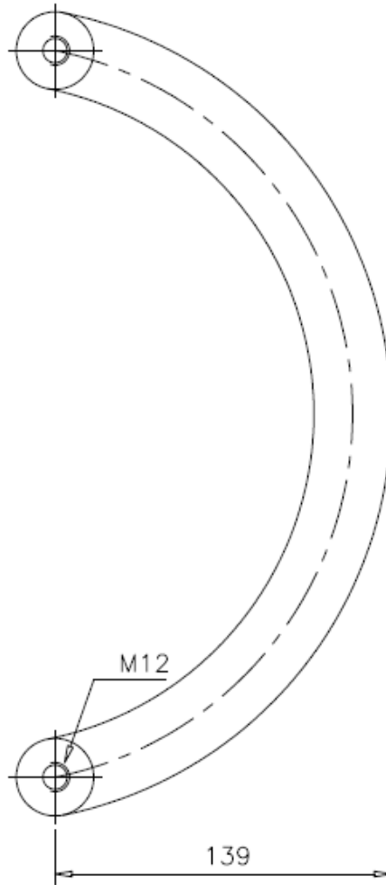
#16.303 Circular Pull # 32 mm diameter x 300 mm M12 threaded for back mounting
